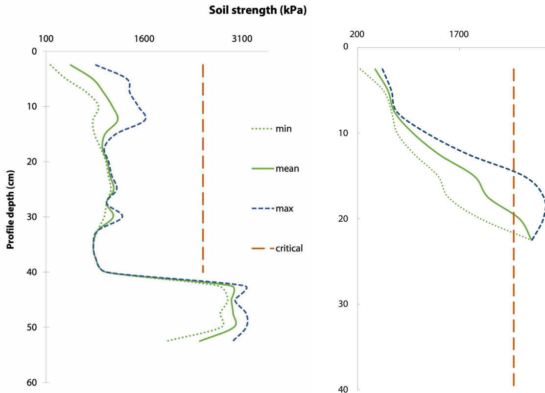
Figure 5. Testing soil strength with a penetrometer and the critical point of 2.5 MPa (2,500 kPa) [Data: Amanda Schapel].
