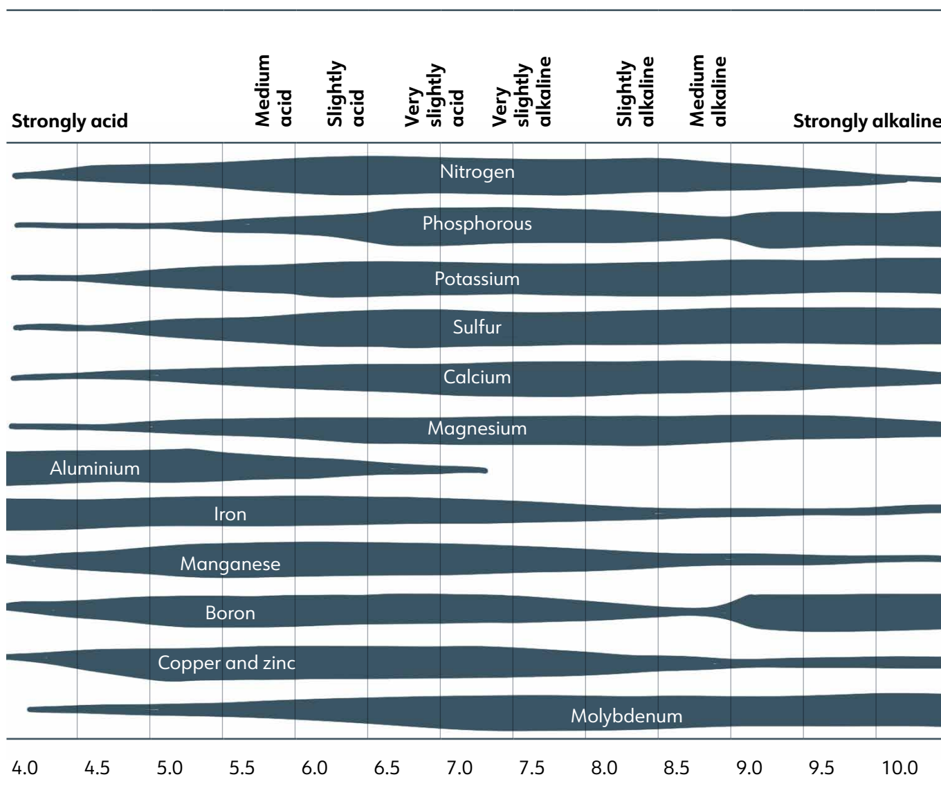
Figure 7. Influence of pH_{water} on nutrient availability (Price, 2006, in Maschmedt, 2004).
